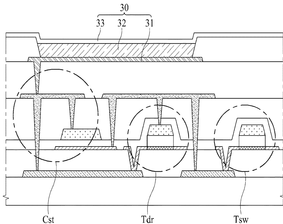
FIG. 1 RELATED ART
